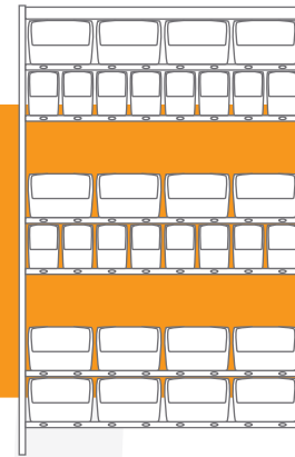
ACTYLUS Smart Bin 8832.6 Max. 6 shelves/48 bins Weight: 67 kg Max. capacity: 261 kg
