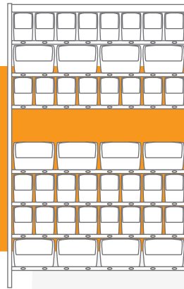
ACTYLUS Smart Bin 8844.7 Max. 7 shelves/56 bins Weight: 74 kg Max. capacity: 305 kg
